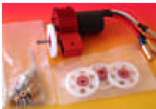
#6615 3850kv, 7.4v, 24x40mm, 100 watt, 2s 10x6 prop, weight 75g and 18 amps. $29.00
